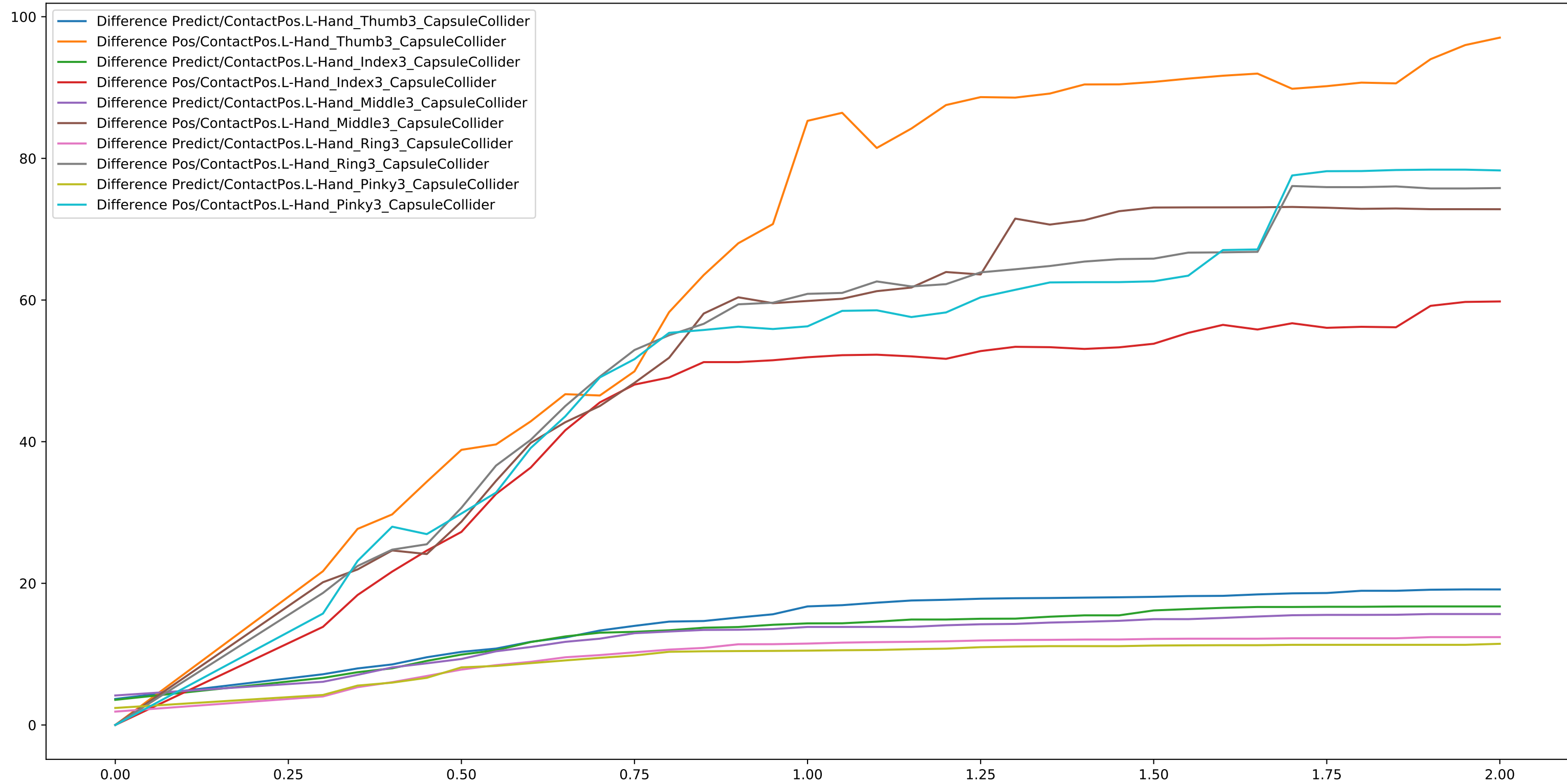
Distance between Prediction and Bones Position to Bone Final Contact Position, function of Time Prediction Known (s), per Phalanx
